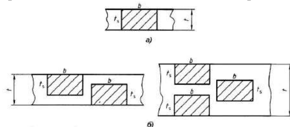
Fig. 6.4.4.1-3 Example showing the position of test specimens in welded joint section:
