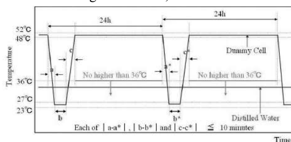
Fig. 2.6.8.1.1.5 Schematic view of temperature controlling accuracy of specimens and distilled water during corrosion test
