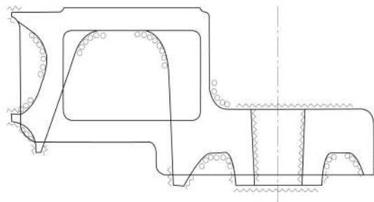
Fig. 2.5.3.3.2-5 Rudder (Upper part). Extent of testing
